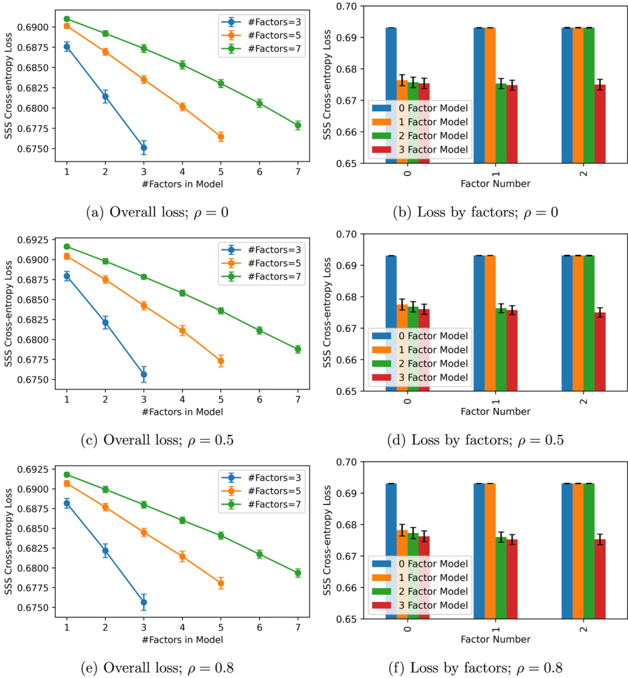
Fig. 2 The three figures on the left show the SSS cross-entropy loss (y-axis) for a class of models in (21), where more relationships are captured progressively (x-axis). The three figures on the right show the SSS cross-entropy loss (y-axis) broken down by factors (x-axis) for a class of models that capture more relationships progressively. The correlation between factors \rho = 0, 0.5, \text{ and } 0.8
