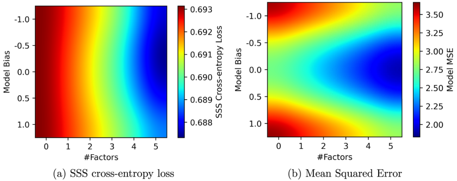
Fig. 3 SSS cross-entropy loss (a) and MSE (b) for a class of models in (22), where more relationships are captured progressively (x-axis), and model bias varies from -1 to 1 (y-axis)
