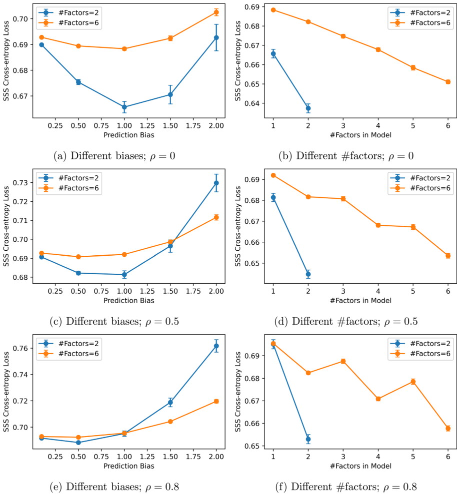
Fig. 1 The three figures on the left show the SSS cross-entropy loss (y-axis) for a class of models in (19), where bias ranges from 0 to 2 (x-axis). The three figures on the right show the SSS cross-entropy loss (y-axis) for a class of models in (20), where more relationships are captured progressively (x-axis). The correlation between factors \rho = 0, 0.5, \text{ and } 0.8
